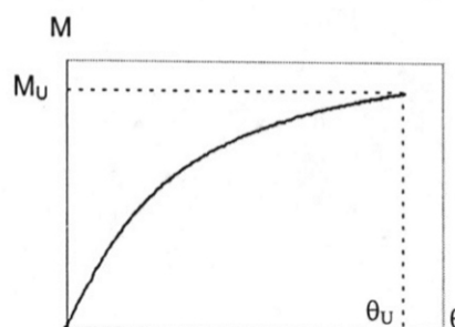
(b) Ultimate moment capacity ( M_U )
