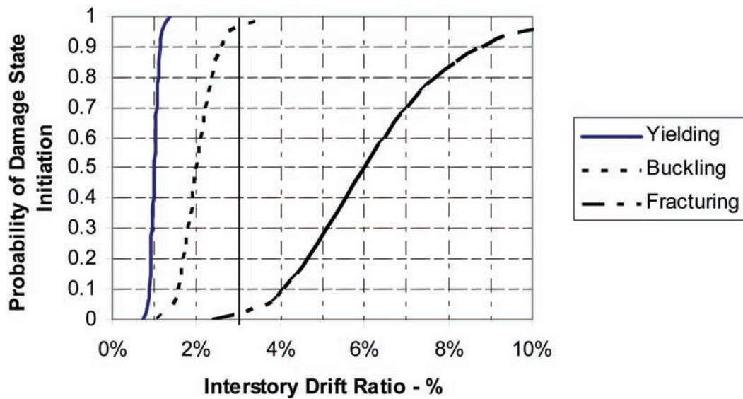
Figure A-10 Example fragility function for beam-column connection behavior.
