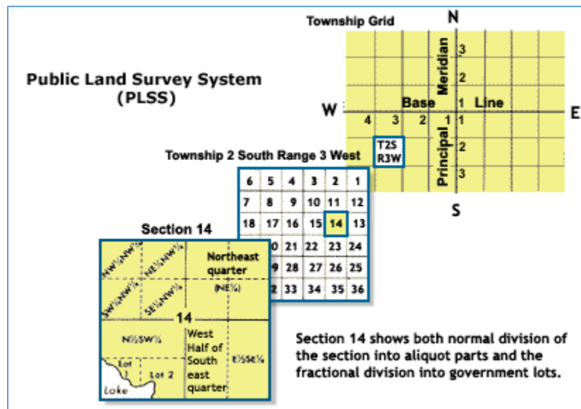
Figure 4: U.S. Public Land Survey System Grid System
