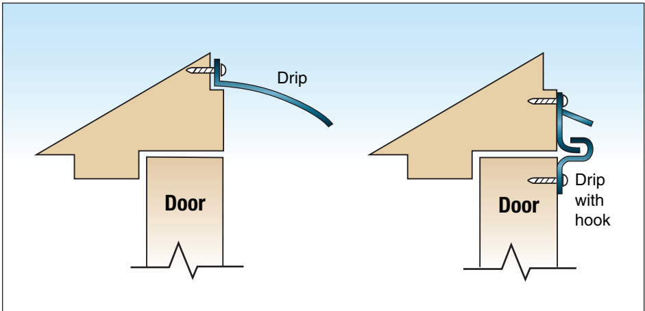
Figure 6-44: Drip at door head and drip with hook at head
