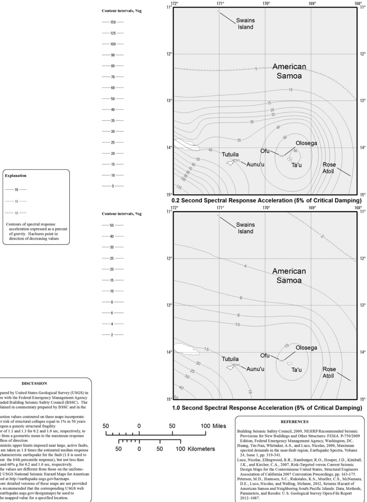
FIGURE 1613.2.1(10) RISK-TARGETED MAXIMUM CONSIDERED EARTHQUAKE ( MCE_R ) GROUND MOTION RESPONSE ACCELERATIONS FOR AMERICAN SAMOA OF 0.2- AND 1-SECOND SPECTRAL RESPONSE ACCELERATION (5% OF CRITICAL DAMPING)
