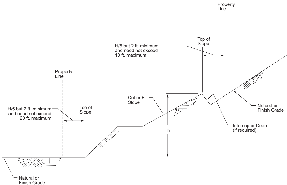
FIGURE J107.3 BENCHING DETAILS
