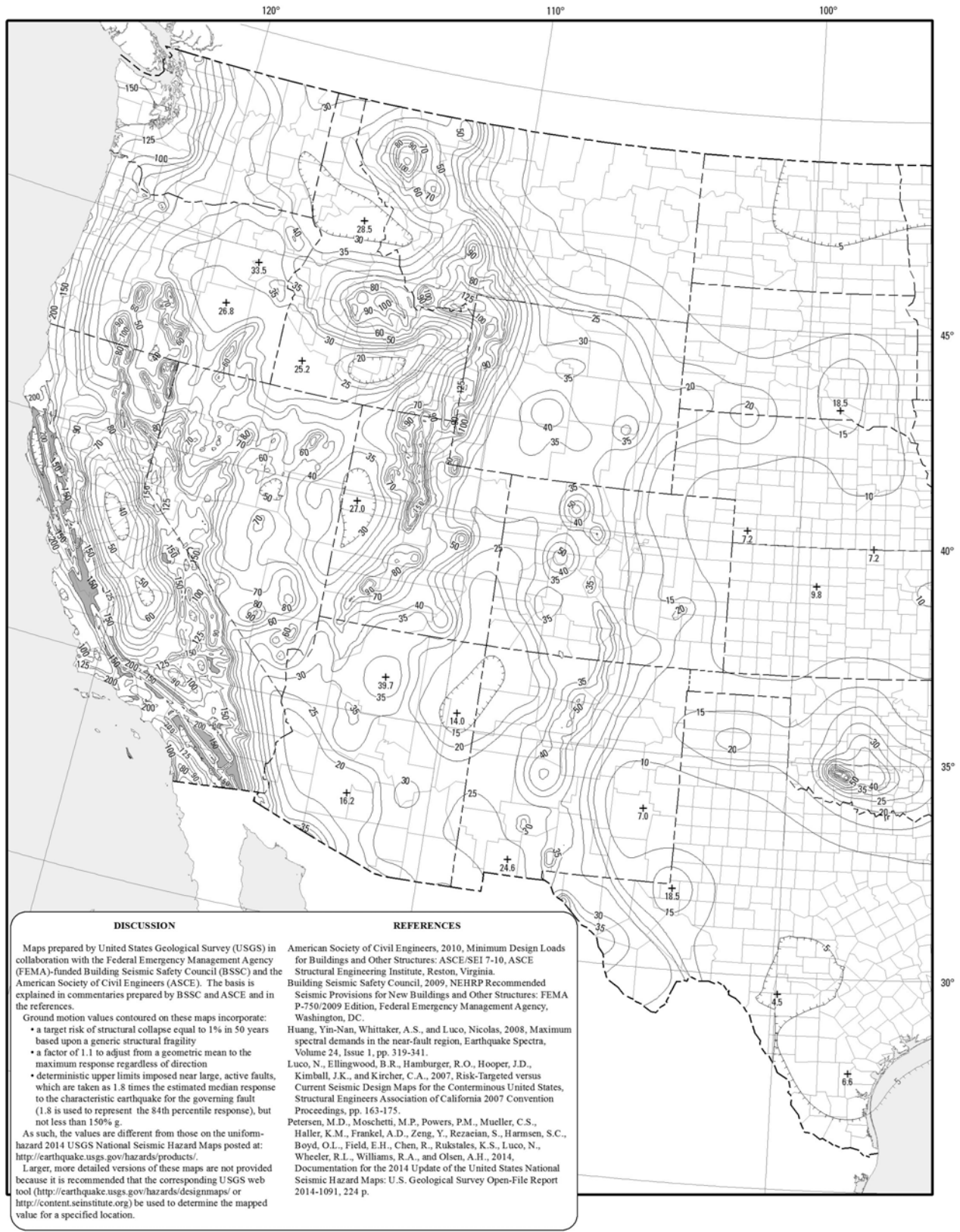
FIGURE 1613.2.1(1) RISK-TARGETED MAXIMUM CONSIDERED EARTHQUAKE ( MCE_E ) GROUND MOTION RESPONSE ACCELERATIONS FOR THE CONTERMINOUS UNITED STATES OF 0.2-SECOND SPECTRAL RESPONSE ACCELERATION (5% OF CRITICAL DAMPING)
